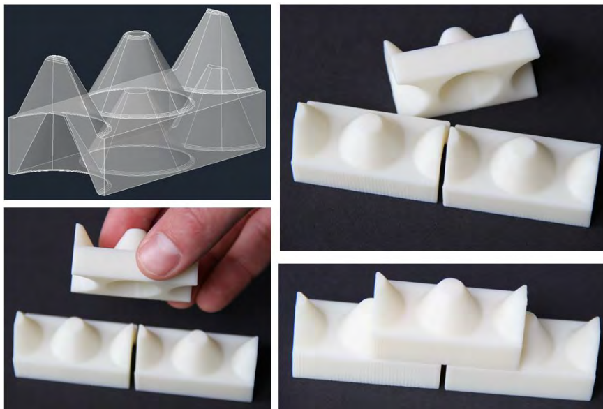
Figure 10: The conical interlocking drick (CID)
