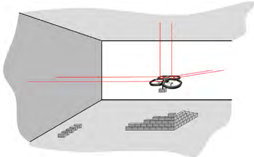
Figure 5: Positioning system based on 3 pairs of lasers
