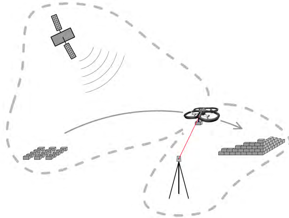
Figure 7: Combination GPS/automatic theodolite
