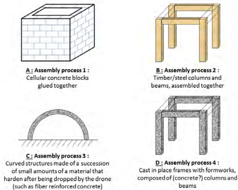
Figure 4: Examples of drone compatible assembly processes (DCAP)
